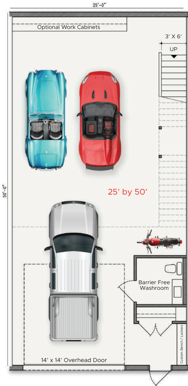
MAIN FRONT BAY 1250 SQ FT
